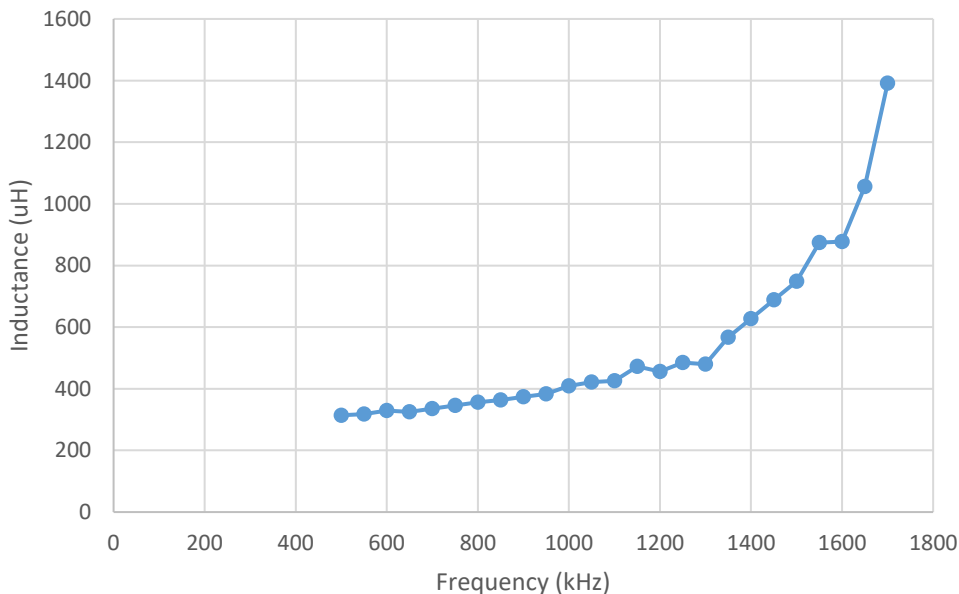
ISO-300-CAT6-2 Inductance (uH) vs. Frequency (kHz)
