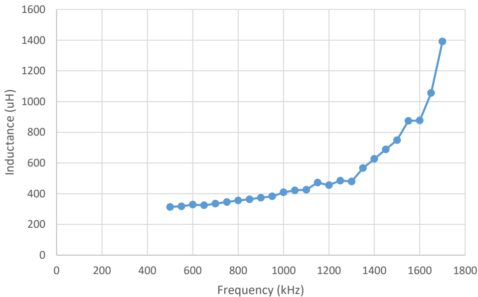
Inductance (uH) vs. Frequency (kHz)
