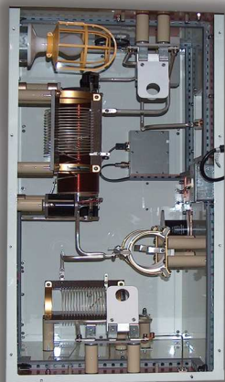
RACK MOUNTABLE LTU MODEL# LTU-1B-RM
