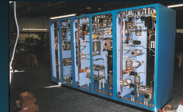
DIRECTIONAL ARRAY PHASING & MATCHING SYSTEMS
