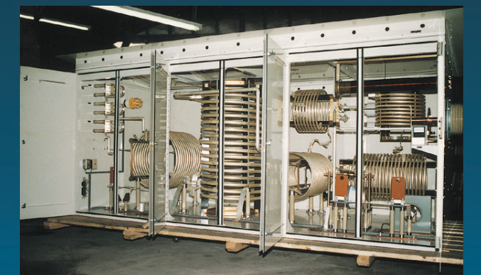
MULTIPLEXED OMNI OR DIRECTIONAL SYSTEMS
