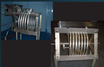
FIXED & VARIABLE INDUCTORS (5-200 AMPS)
