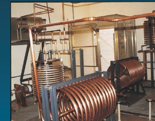
DIRECTIONAL ARRAY FEEDER SYSTEMS
