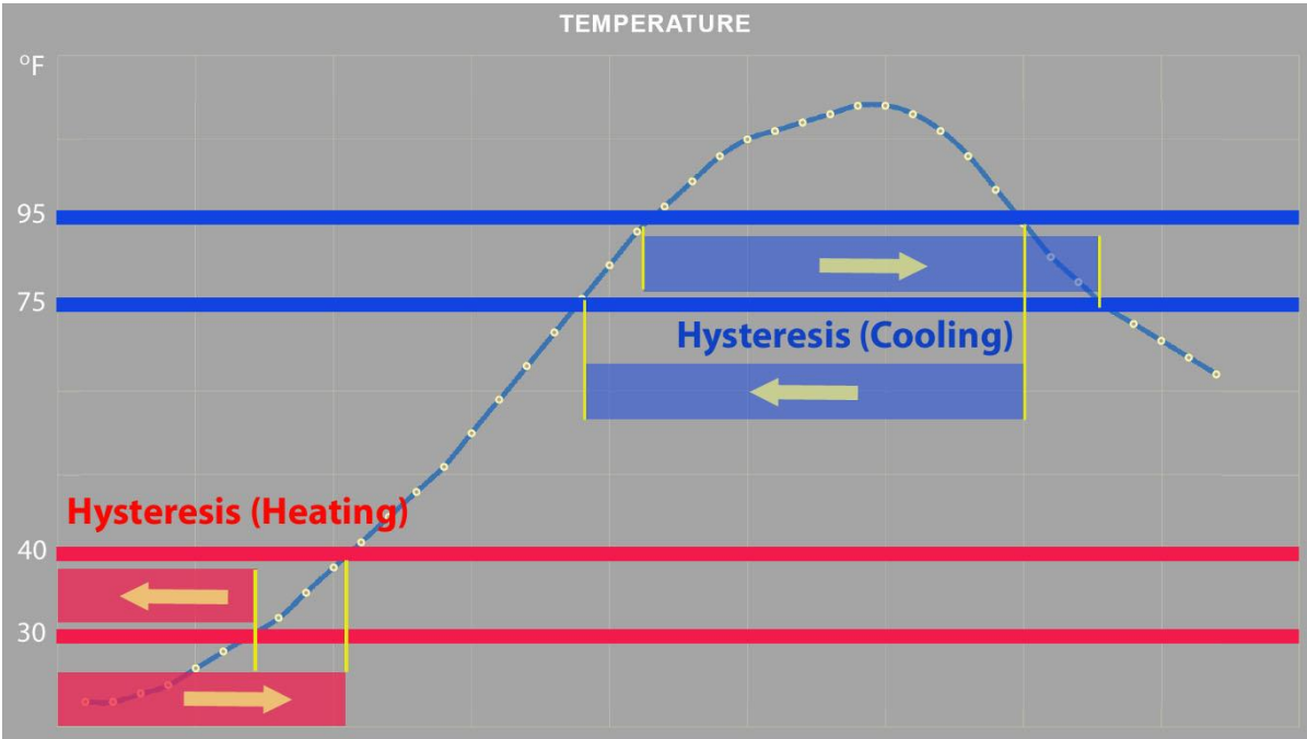
Fig. 3 Hysteresis – KTL factory settings
