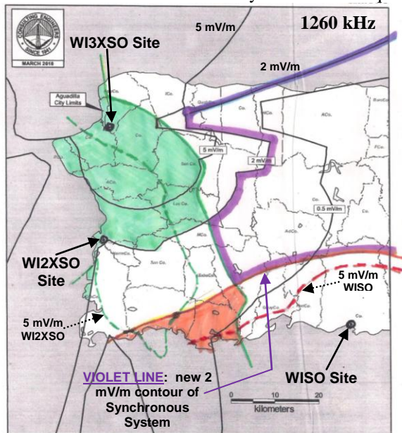
FIGURE 9 — PREDICTED COVERAGE CONTOURS OF WISO AND ITS WI2XSO AND WI3XSO SYNCHRONIZED BOOSTERS
