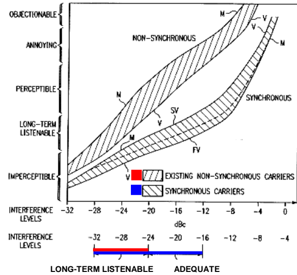
FIGURE 1 – AUDIBILITY OF CO-CHANNEL FRINGE BEATS
