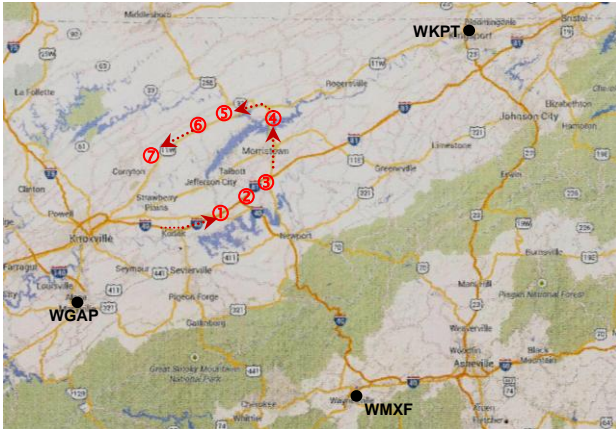
FIGURE 8. MAP SHOWING THE LOCATIONS OF THE TWO TEST AM STATIONS AND THE MONITORING LOCATIONS
