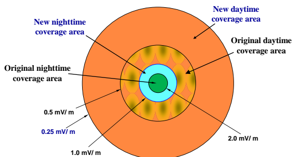
FIGURE 15 — EFFECTIVE SYNCHRONOUS DAY/NIGHT INTERFERENCE-LIMITED COVERAGE IMPROVEMENTS
