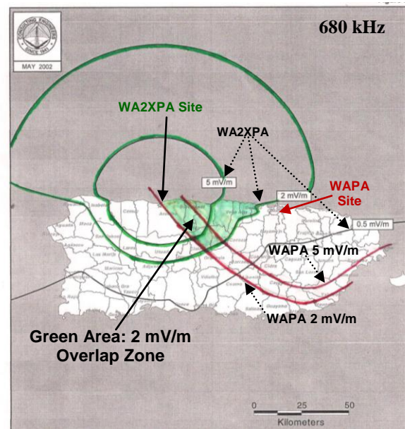
FIGURE 10 — PREDICTED COVERAGE CONTOURS OF WAPA AND ITS WA2XPA SYNCHRONIZED BOOSTER
